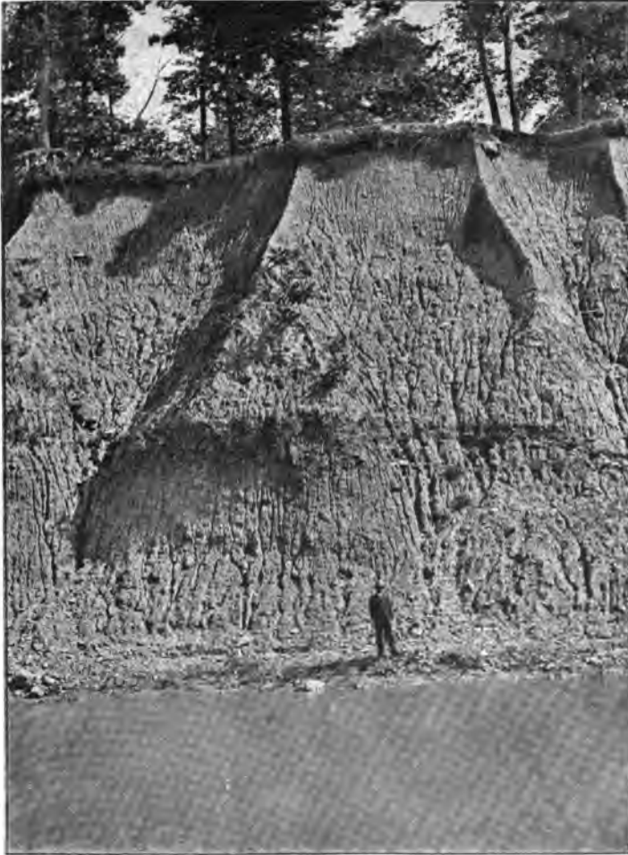
FIG. 118.—Section in till near Darrown, Butler County, Ohio, sixty-five feet high. Coarse line of stratification near the middle. Fresh cedar logs at the bottom. (See text.) (United States Geological Survey.) (Wright.)
